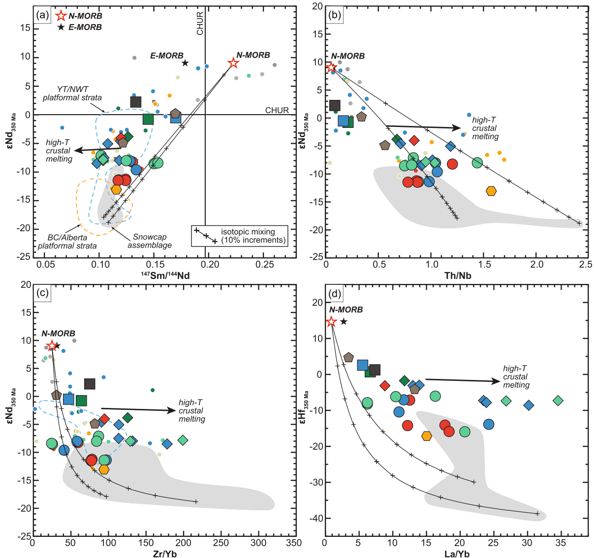
FIGURE 17: Isotope and trace element ratio mixing curves: (a) \epsilon\text{Nd}_{350 \text{ Ma}} vs. ^{147}\text{Sm}/^{144}\text{Nd} ; (b) \epsilon\text{Nd}_{350 \text{ Ma}} vs. \text{Th}/\text{Nb} ; (c) \epsilon\text{Nd}_{350 \text{ Ma}} vs. \text{Zr}/\text{Yb} ; (d) \epsilon\text{Hf}_{350 \text{ Ma}} vs. \text{La}/\text{Yb} . Endmembers are N-MORB (star), using trace element values from Sun and McDonough [91] and depleted mantle isotopic compositions as in Figure 15, and Snowcap assemblage (grey region; [5, 157, 158]). Dashed lines indicate location of samples from platformal strata of the North American ancestral margin from Yukon-Northwest Territories (blue; [159]) and BC-Alberta (orange; [160]). Graticules on mixing curves are shown as 10% increments. Symbols and colors as in Figure 10. Data that fall significantly off the mixing curves are interpreted to be results of high-temperature crustal melting (see text for details).
